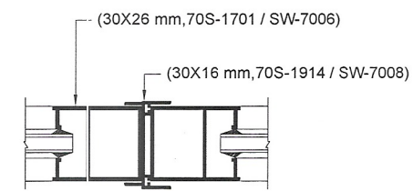
SECTION - A
