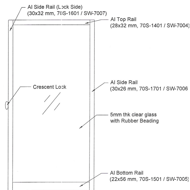
Window Sash
