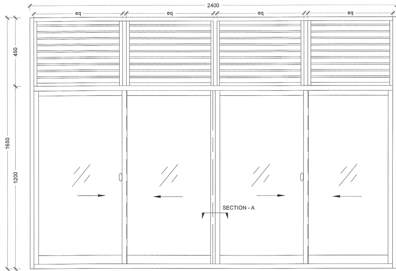
Window Front
