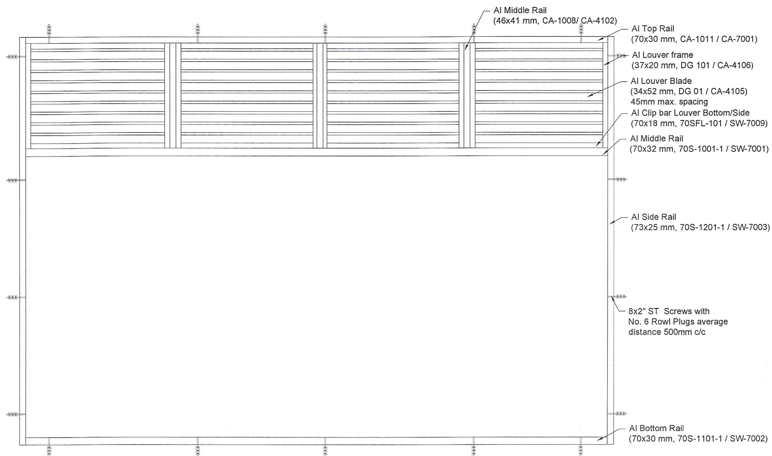
Window Frame
