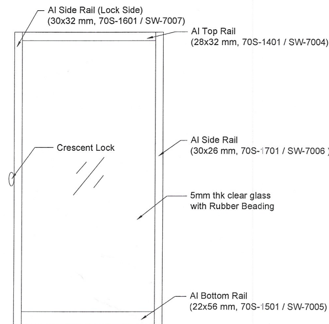
Window Sash
