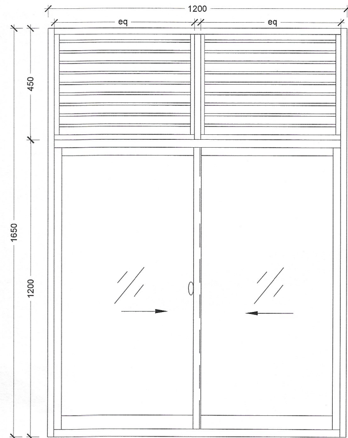
Window Front
