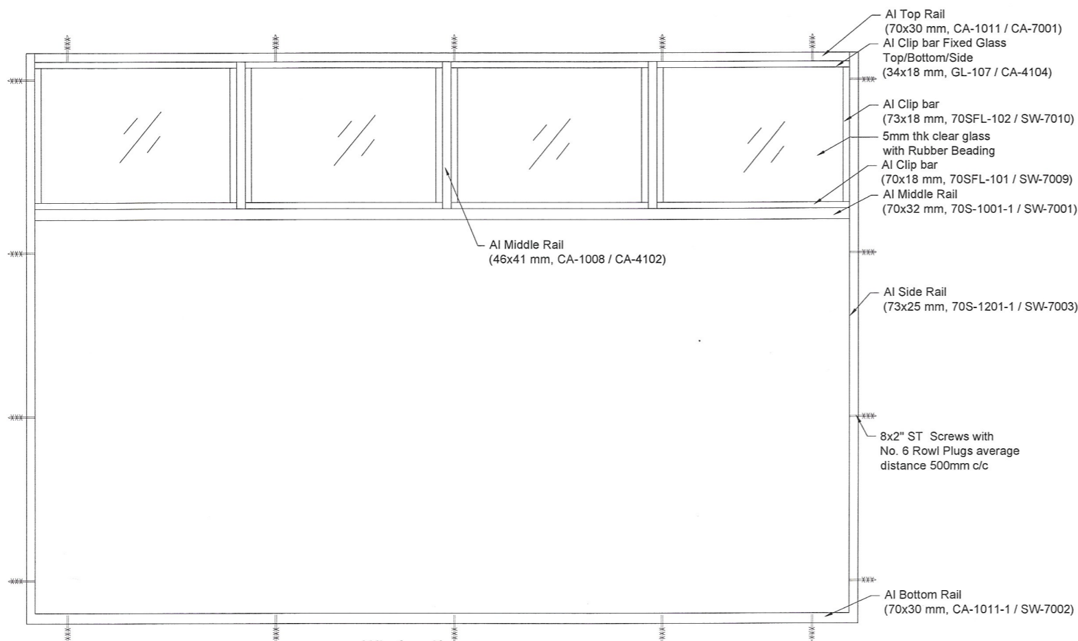
Window Frame
