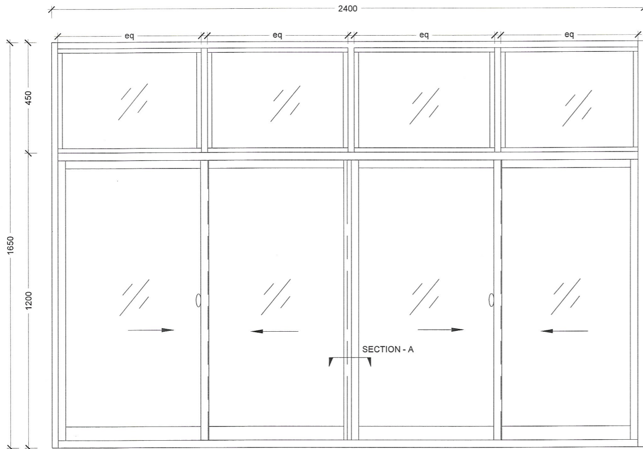
Window Front
