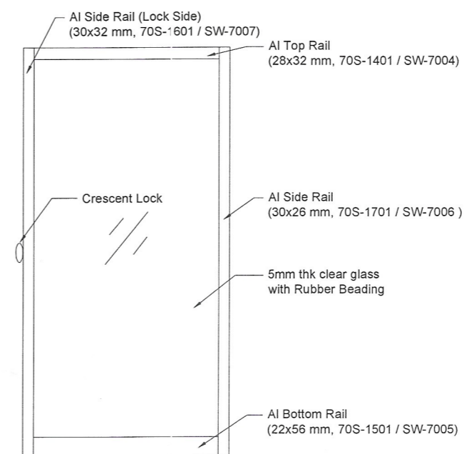
Window Sash
