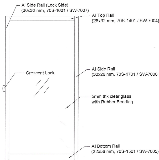
Window Sash
