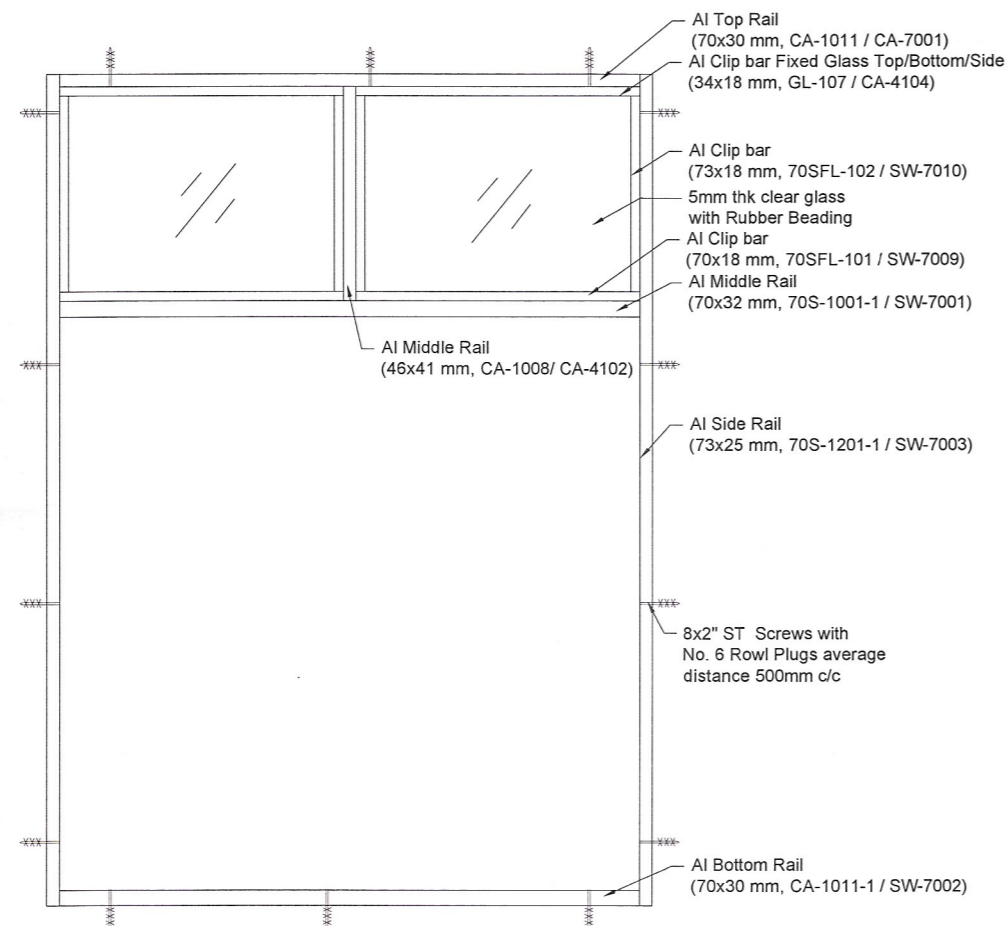
Window Frame
