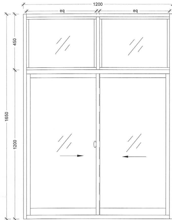
Window Front
