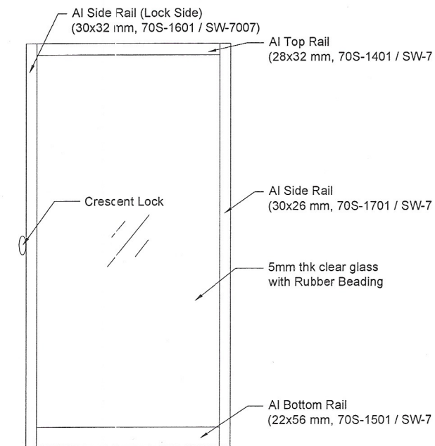
Window Sash
