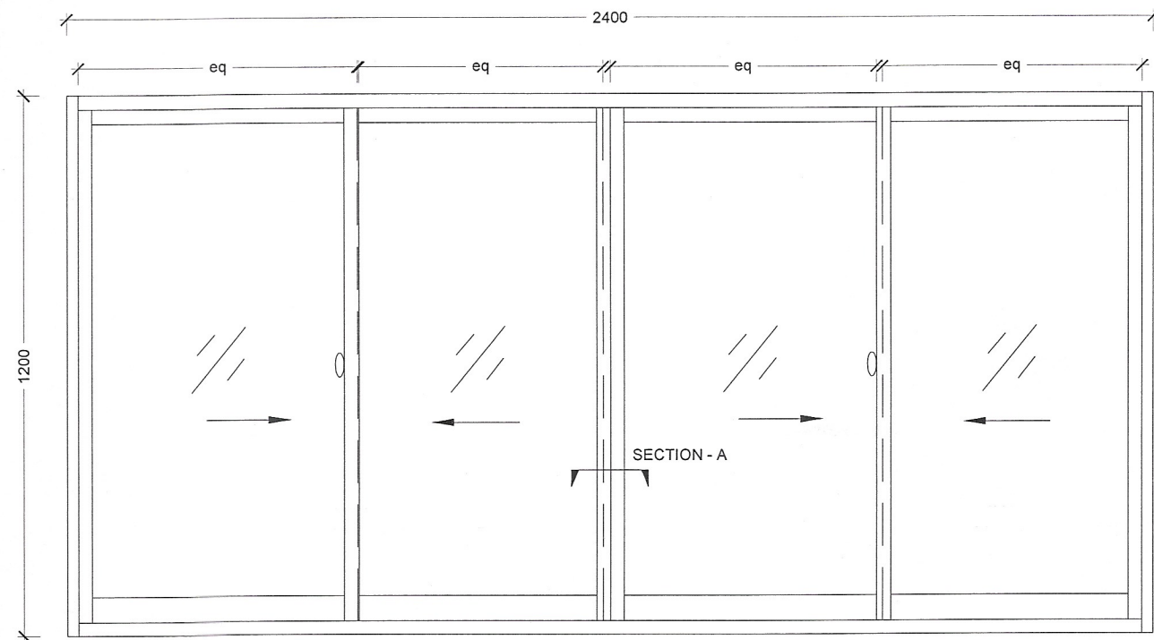
Window Front
