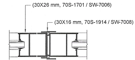
SECTION - A
