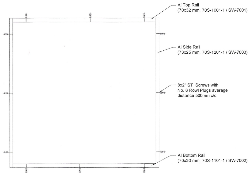
Window Frame
